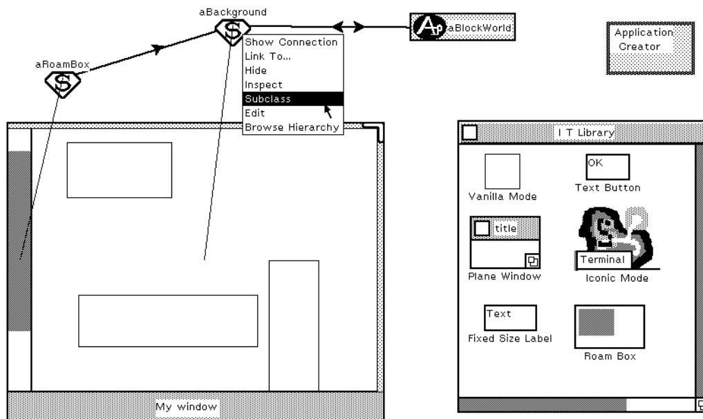
Figure 1.1: Using MoDE.
